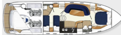
Upper accommodation layout
